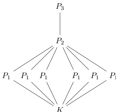
FIGURE 1. The P groups: K \triangleleft P_1, P_2, P_3 and P_2 \triangleleft P_3 . The group P_1 occurs six times as a subgroup of P_2 (a single conjugacy class), i.e., as G_{q_1, q_2} , q_1 \neq q_2 , q_1, q_2 \in \{i, j, k\} .
