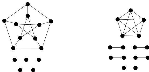
FIG. 1.1. The graph drawn on the left is a graph non-isomorphic to a disjoint union of complete graphs but Laplacian cospectral with the disjoint union of complete graphs drawn on the right
